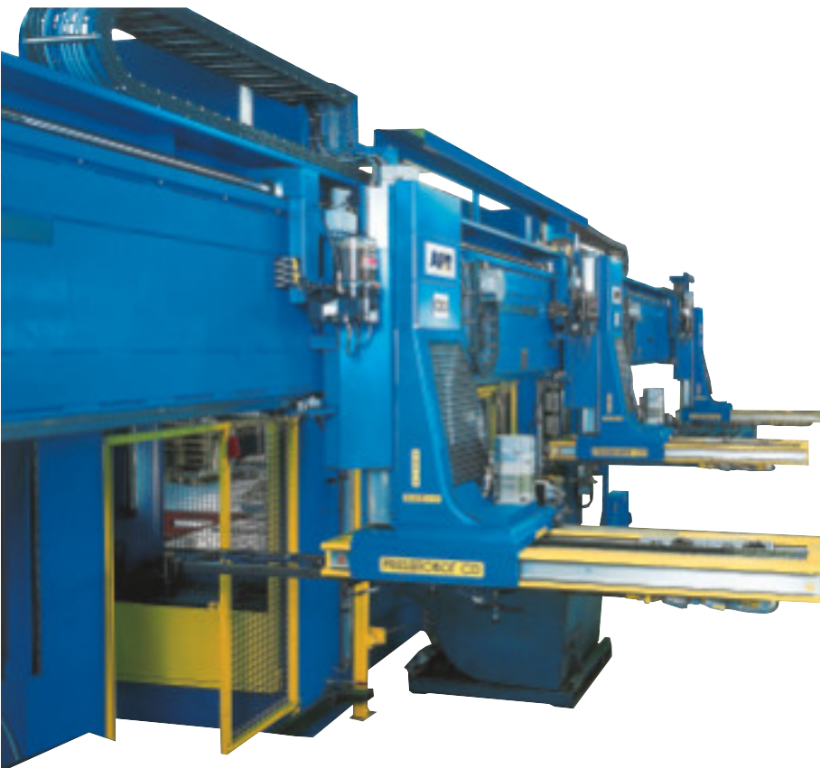
AP&T Pressline 3 x 5 000 kN. Hydraulic press operated by CD robots.
