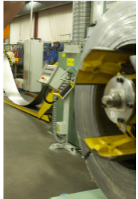
SMV Automatic presses 1 250 kN with Dimeco belt conveyor.
